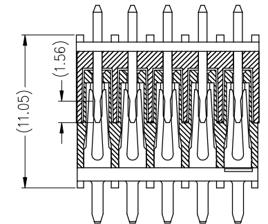
Female&Male mating
