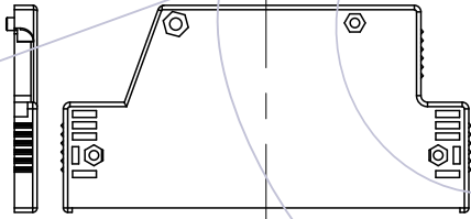
56P BOTTOM COVER
