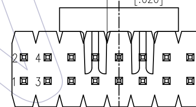
Dual Numbers
