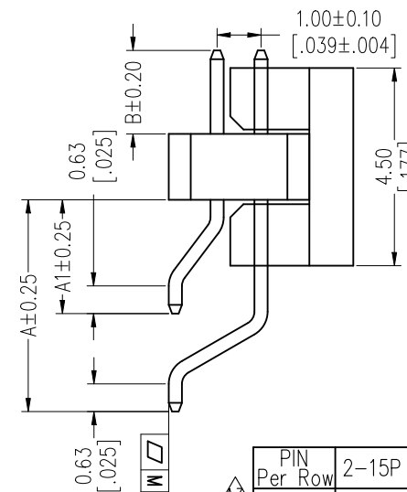
Dual Numbers
