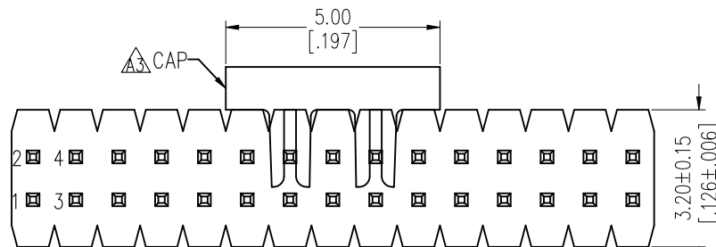
Odd Numbers
